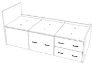
MB044 - 3 Drawer Bed with Lifting Void 1950(L) x 800/950(W) x 519(H)
